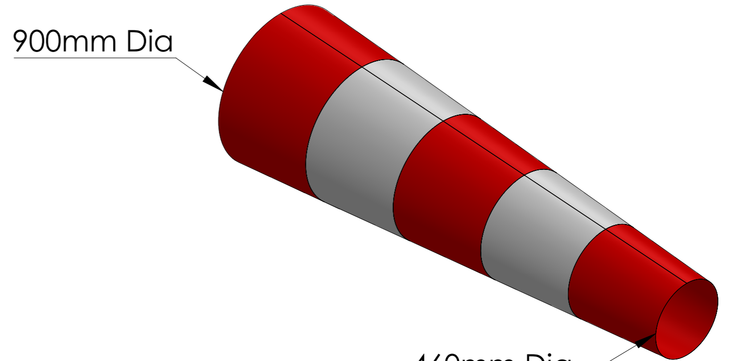
ISOMETRIC VIEW
