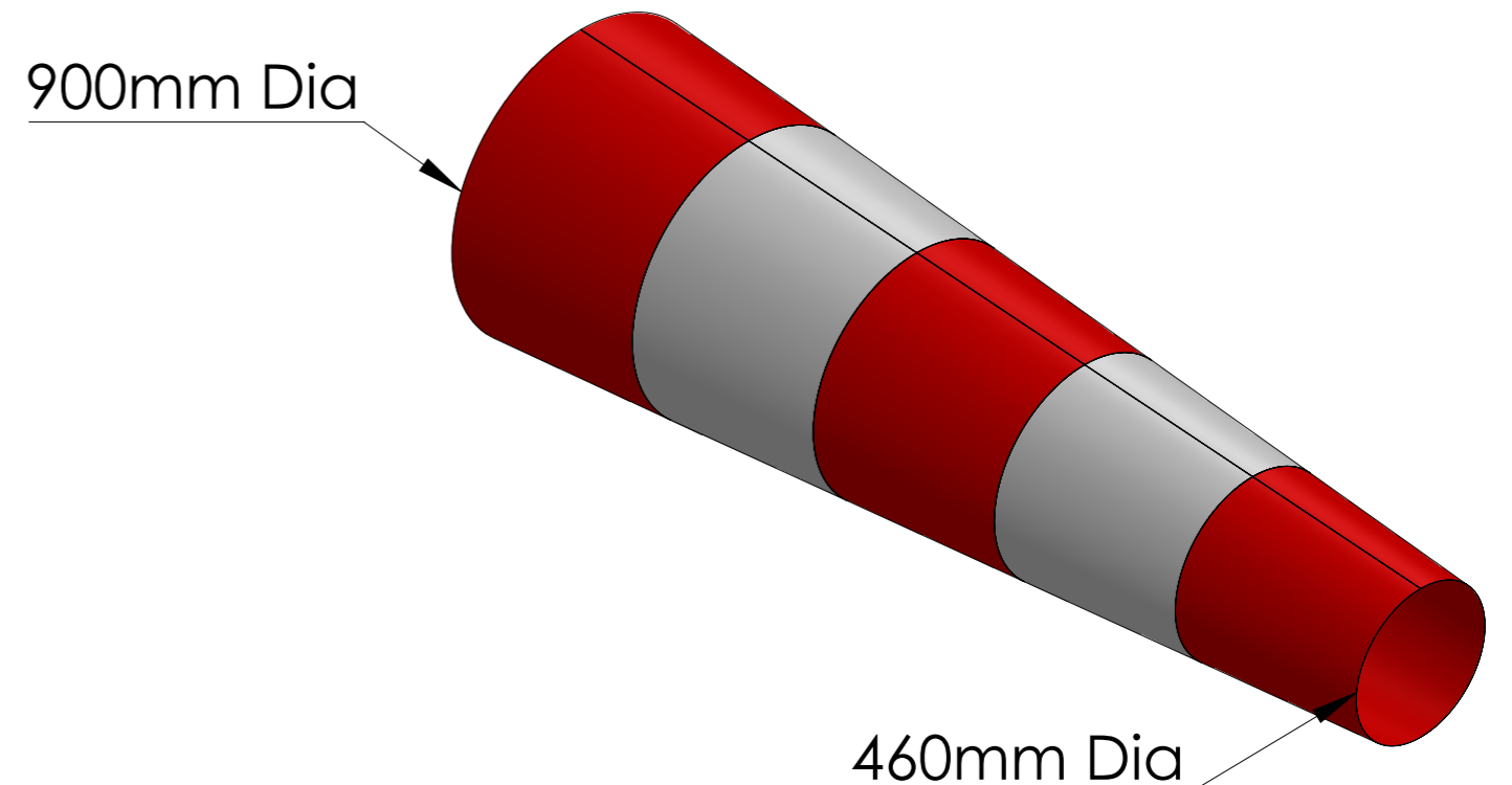
ISOMETRIC VIEW
