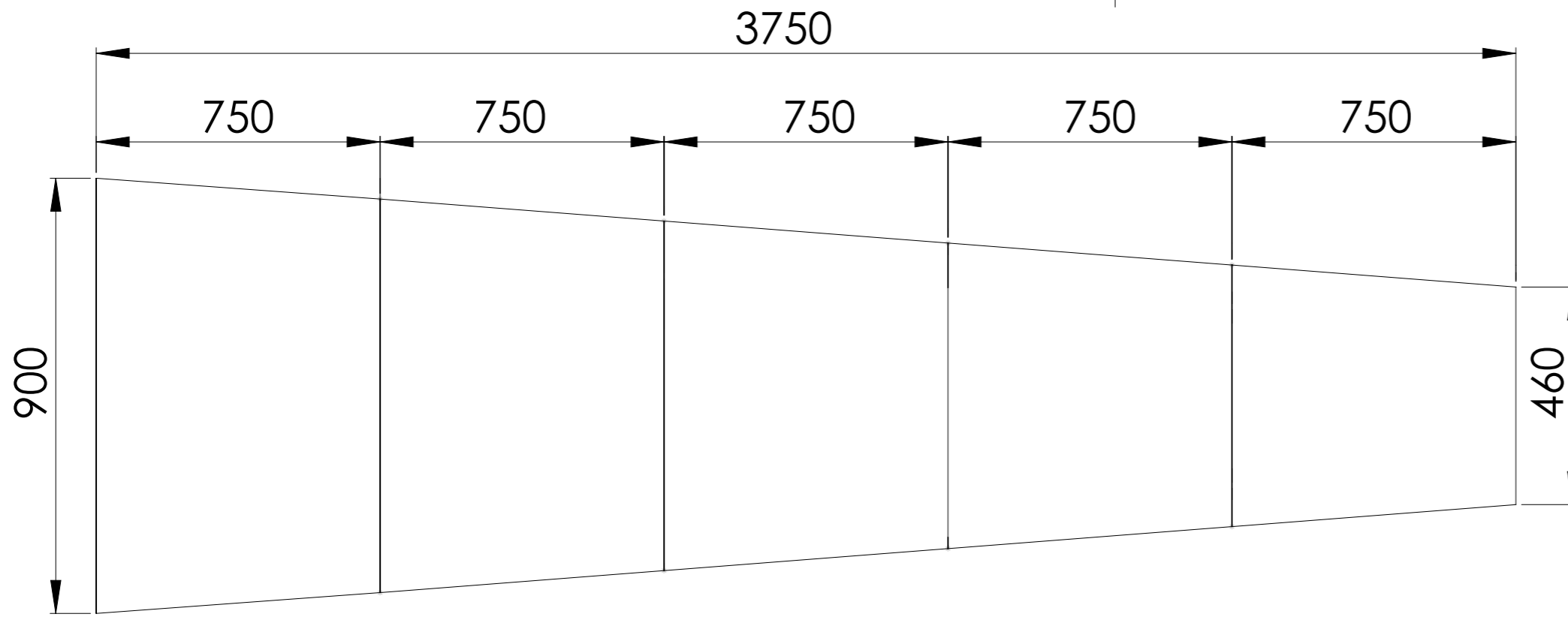
FRONT VIEW
