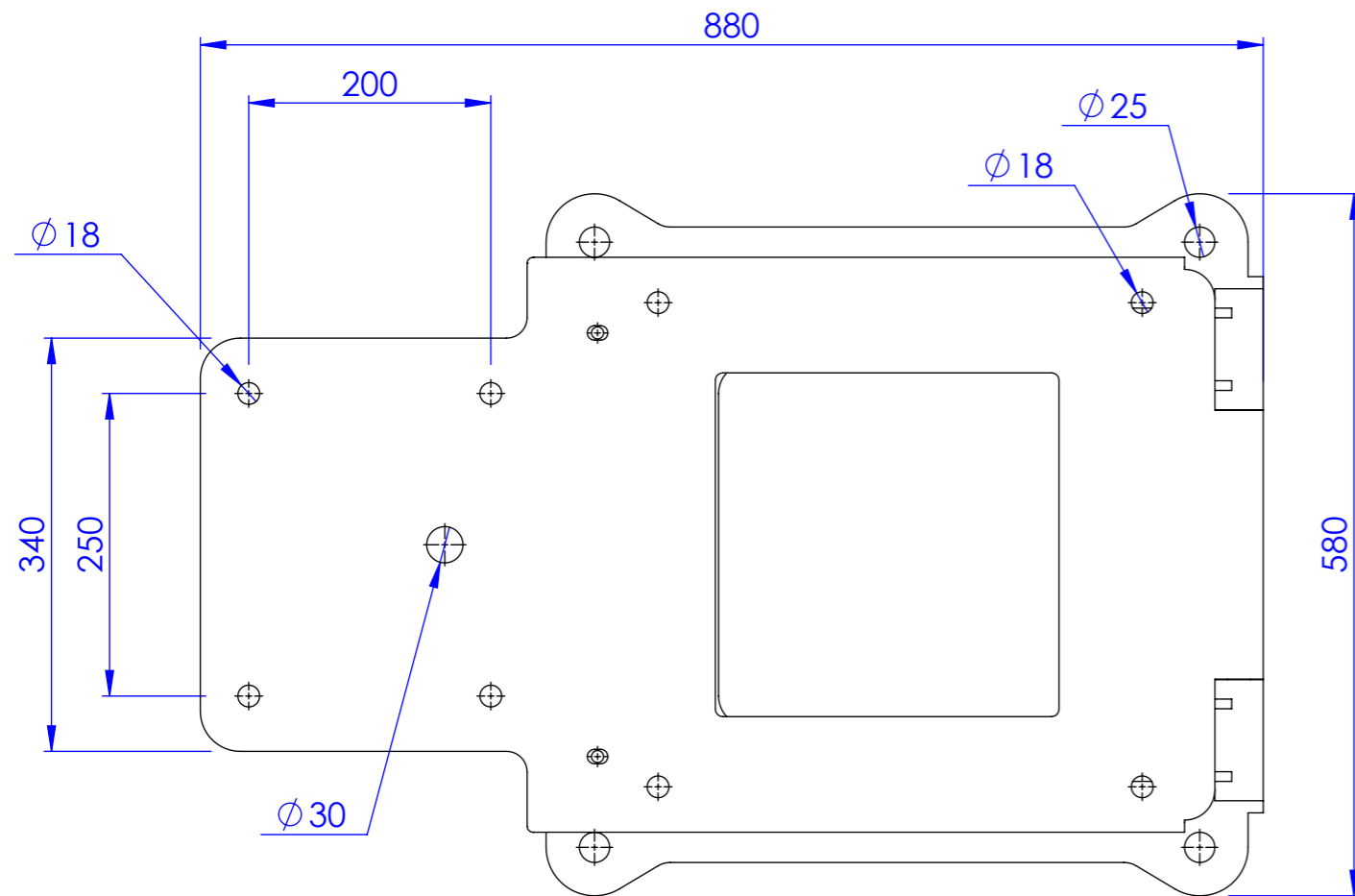
TOP VIEW
